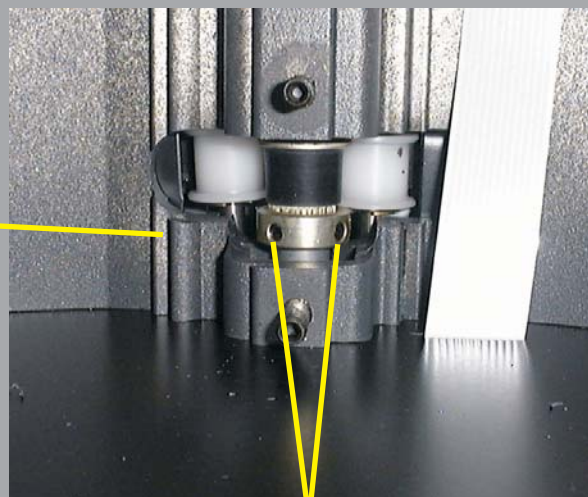
Setscrews
